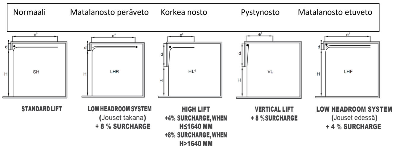
Dimensions for sectional door IDO-PRO (mm)
